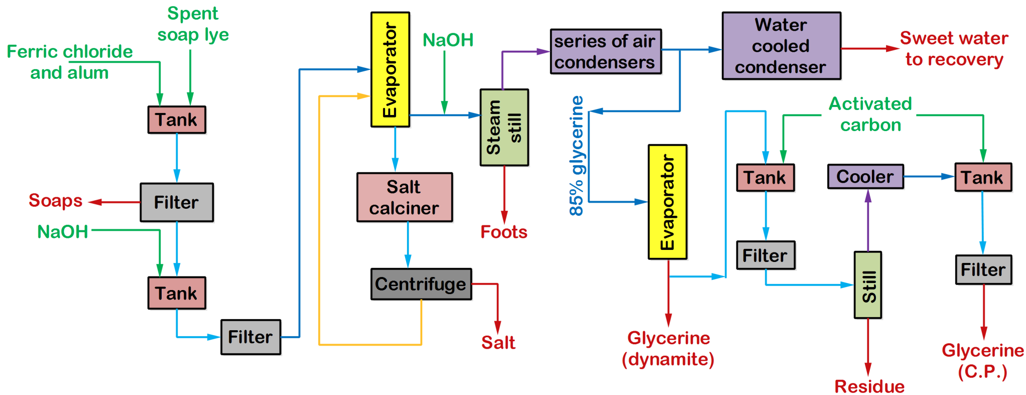
Figure: Manufacture of glycerol from soap
